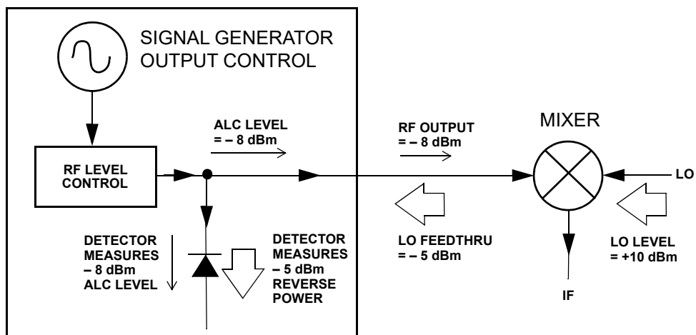
Effects of Reverse Power on ALC
