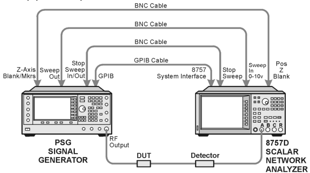
Figure 2-3 Equipment Setup
