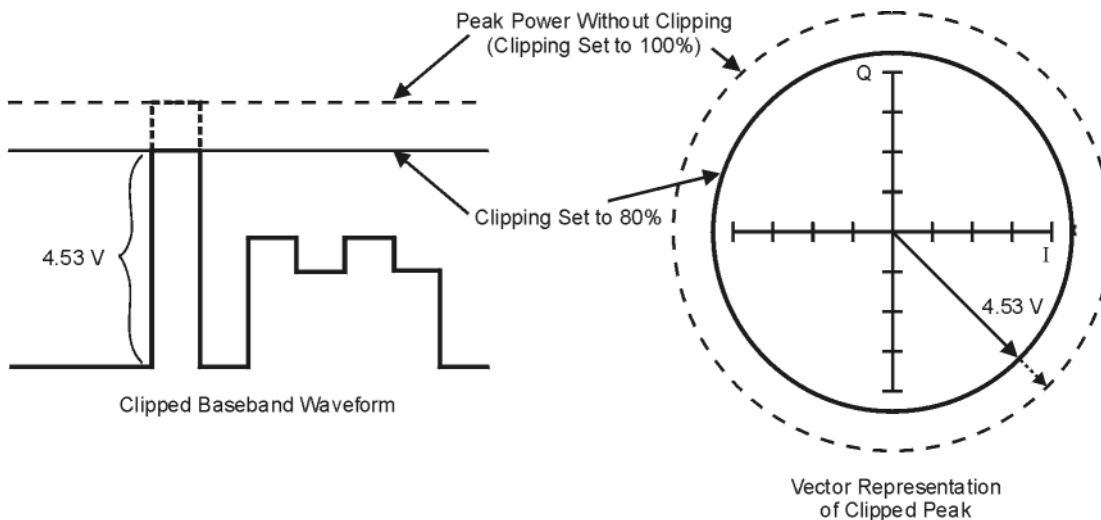
Figure 3-15 Rectangular Clipping
