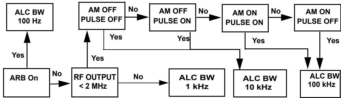
Figure 4-1 Decision Tree for Automatic ALC Bandwidth Selection
