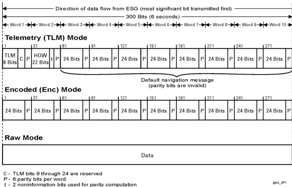
Figure 8-4 Subframe Structures
