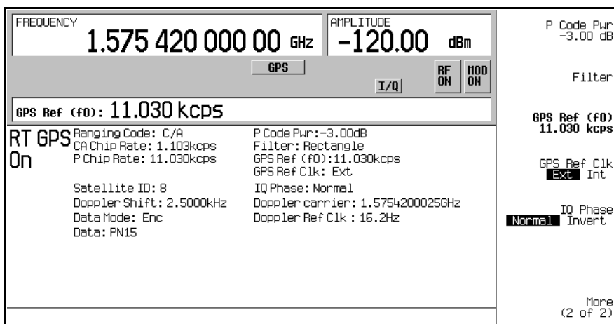
Real Time GPS Setup with External Clock
